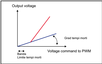
Dead time compensation
